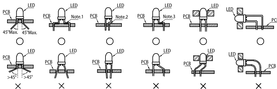
" ○ " Correct mounting method " × " Incorrect mounting method
